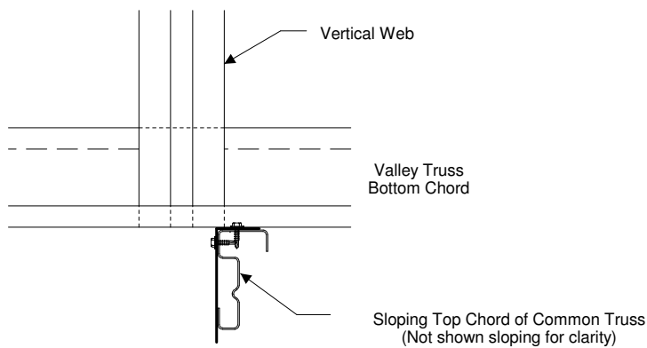
Section X-X
